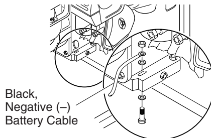
Figure 11 - Connecting Black, Negative (-) Battery Cable to Engine Block (Model MGH6500IE Shown)
